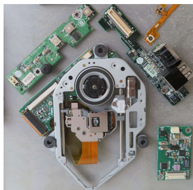
The CD drive, disassembled
